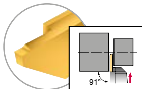
CD8 chip breaker geometry for parting off
