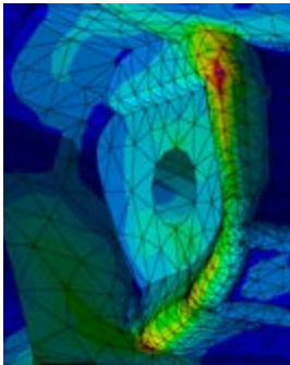
FEM analysis: improved stability through reduced deformation under load
