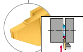
RA8 chip breaker geometry for radius grooving
