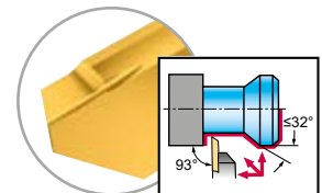
DG8 chip breaker geometry for forward turning
