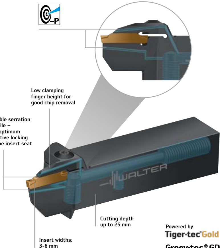
Axial grooving tool with Precision cooling
